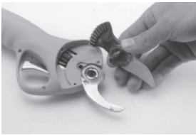
4. Unscrew the pin and remove the moving blade
